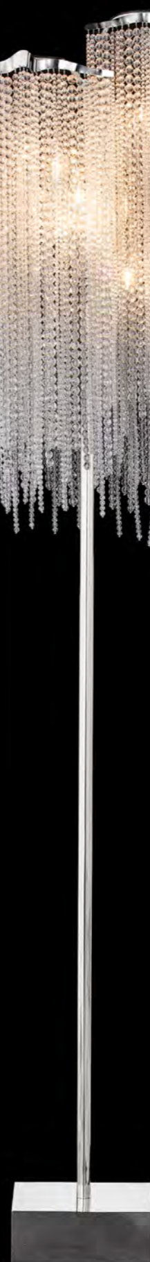
VF190N Victoria Floor Lamp (Ø30xH.190 cm, nickel finish, 5 x E14, 27 kg) Technical details page 310
